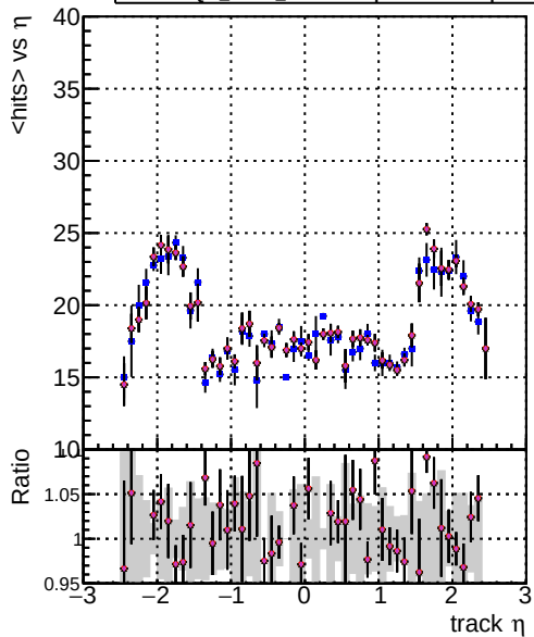
mean hit DOM CKE Tbar DOM mkFit TbarPU-updated DOM mkFit TbarPU-updated-newPLDNN-2 DOM mkFit TbarPU-updated-DNNSqcd13
