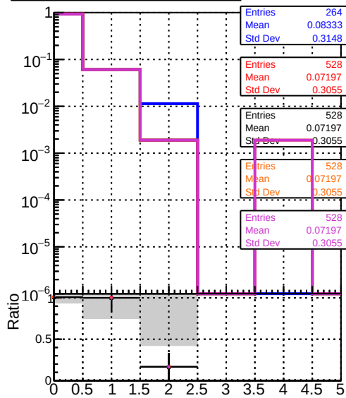
mean hit DOM CKE Tbar DOM mkFit TbarPU-updated DOM mkFit TbarPU-updated-newPLDNN-2 DOM mkFit TbarPU-updated-DNNSqcd13
