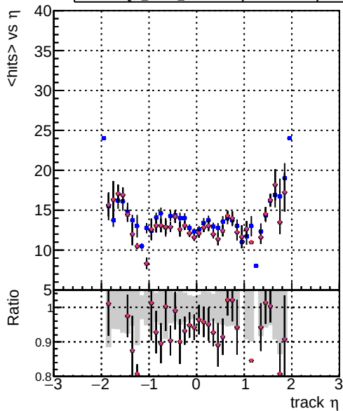
mean hit DOM_CKE_TTbar DOM_mkFit_TTbarPU-updated DOM_mkFit_TTbarPU-updated-newPLDNN-2 DOM_mkFit_TTbarPU-updated-newPLDNN-2 DOM_mkFit_TTbarPU-updated-DNNsgc113
