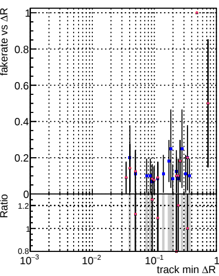
Fake rate vs \Delta R(\text{track, jet}) Legend: DQM, CKF, Tthor, PU-updated, newPLDNN, DNNsqc013
