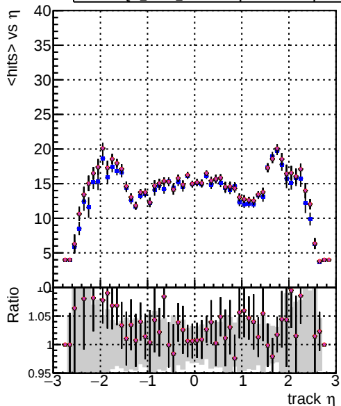
mean hit DOM_CKE_TTbar DOM_mkFit_TTbarPU-updated DOM_mkFit_TTbarPU-updated-newPLDNN-2 DOM_mkFit_TTbarPU-updated-newPLDNN-2 DOM_mkFit_TTbarPU-updated-DNNsgcd13
