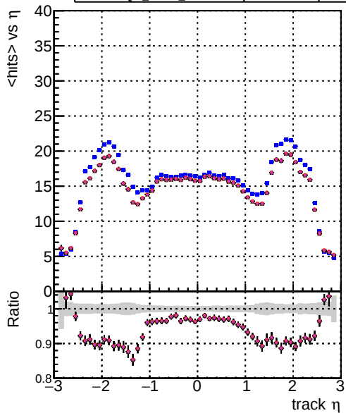
mean hit DOM_CKE_TTbar DOM_mkFit_TTbarPU-updated DOM_mkFit_TTbarPU-updated-newPLDNN DOM_mkFit_TTbarPU-updated-newPLDNN-2 DOM_mkFit_TTbarPU-updated-DNNsgcd13
