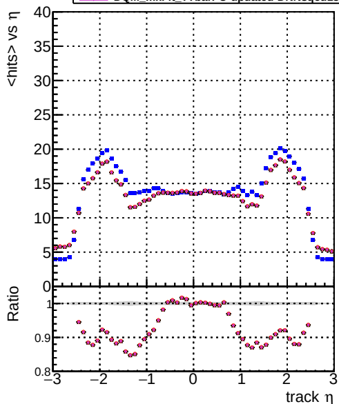
mean hit DOM CKE Tbar DOM mkFit TbarPU-updated DOM mkFit TbarPU-updated-newPLDNN-2 DOM mkFit TbarPU-updated-newPLDNN-2 DOM mkFit TbarPU-updated-DNNSqcc13
