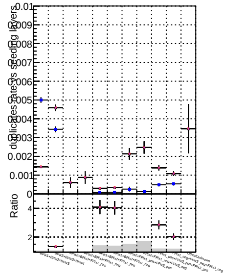
newBLDNN DNNsqcd13-2
