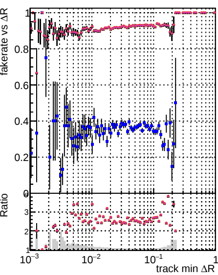
Fake rate vs \Delta R(\text{track, jet}) Legend: BQM GKF TThor PU-updated newPLDNN_2 DNNsqcd13
