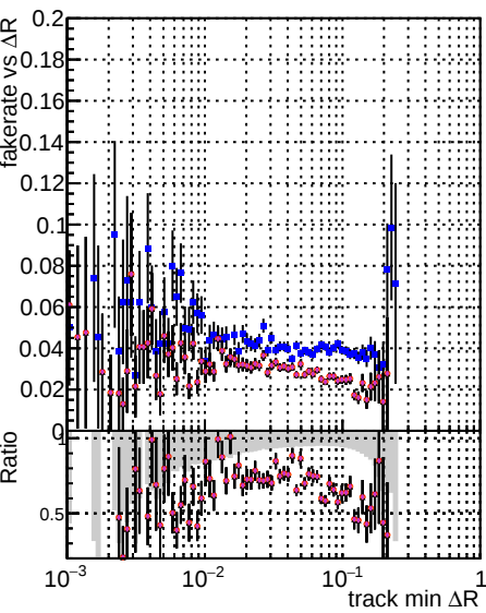
Fake rate vs \Delta R(\text{track, jet}) DQM CKF Tthor DQM+PU DQM+PU+updated CKF+PU CKF+PU+updated Tthor+PU Tthor+PU+updated newPLDNN_2 newPLDNN_2+sqcd13
