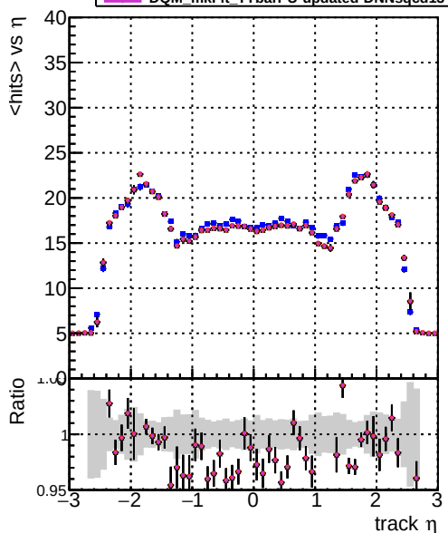
DOM CKE T1bar DOM mkFit T1barPU-updated DOM mkFit T1barPU-updated-newPLDNN DOM mkFit T1barPU-updated-newPLDNN-2 DOM CKE T1bar DOM mkFit T1barPU-updated DOM mkFit T1barPU-updated-newPLDNN-2
