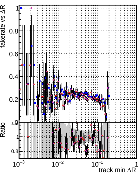
Fake rate vs \Delta R(\text{track, jet}) Legend: DQM (black), CKE (blue), TTher (red), PU-updated (green), newPLDNN_2 (purple), newPLDNN_1 (orange), newPLDNN_3 (yellow), newPLDNN_4 (pink), newPLDNN_5 (brown), newPLDNN_6 (gray), newPLDNN_7 (light blue), newPLDNN_8 (light green), newPLDNN_9 (light red), newPLDNN_10 (light orange), newPLDNN_11 (light yellow), newPLDNN_12 (light pink), newPLDNN_13 (light brown).
