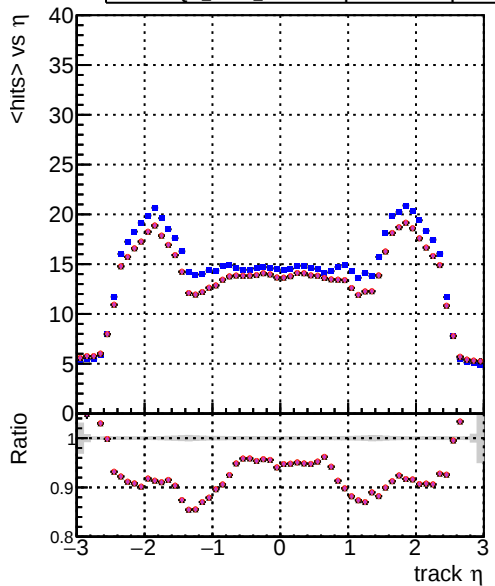
mean hits DOM CKE Tbar DOM mkFit TbarPU-updated DOM mkFit TbarPU-updated-newPLDNN-2 DOM mkFit TbarPU-updated-newPLDNN-3 DOM mkFit TbarPU-updated-DNNsqcd
