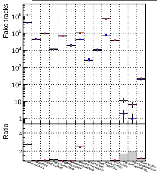
Number Legend Model 1 Blue square DOM_CKE_TTbar 2 Red circle DOM_mkFit_TTbarPU-updated 3 Black triangle DOM_mkFit_TTbarPU-updated-newPLDNN 4 Orange star DOM_mkFit_TTbarPU-updated-newPLDNN-2 5 Green plus DOM_mkFit_TTbarPU-updated-TTbarDNN
