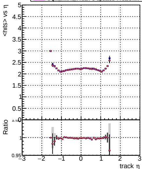
mean hits vs \eta Legend: DOM_CKE_TTbar DOM_mkFit_TTbarPU-updated-newPLDNN DOM_mkFit_TTbarPU-updated-newPLDNN-2 DOM_mkFit_TTbarPU-updated-TTbarDNN DOM_mkFit_TTbarPU-updated-TTbarDNN
