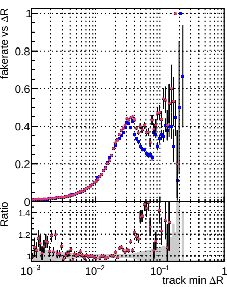
Fake rate vs \Delta R (track, jet) for DQM, CKF, Tthor, PU-updated-new, PU-updated-newBLDNN-2, PU-updated-newBLDNN-2
