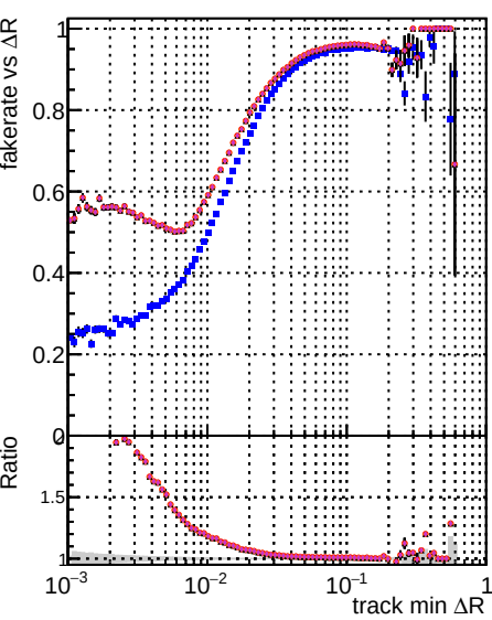
Fake rate vs \Delta R(\text{track, jet}) DQM CKF Tthor Tthor PU-updated newB-DNN-2 Tthor PU-updated-newB-DNN-2
