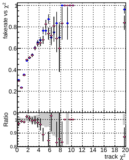
Fake rate vs. DOM GKE TTbar DOM GKE TTbar BU-updated newBLDNN-2 DOM GKE TTbar BU-updated newBLDNN-2
