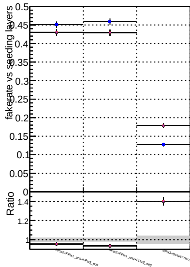
Fake rate vs. DOM CKE TThor TThorBU new R1DNN-2
