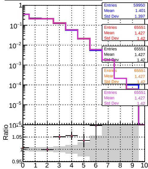
mean hits vs \eta DOM_CKE_TTbar DOM_mkFit_TTbarPU-updated DOM_mkFit_TTbarPU-updated-newPLDNN DOM_mkFit_TTbarPU-updated-newPLDNN-2 DOM_mkFit_TTbarPU-updated-TTbarDNN
