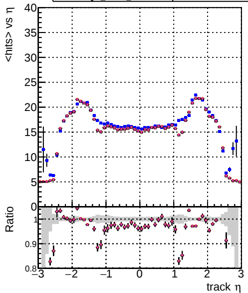
DOM_CKE_TTbar DOM_mkFit_TTbarPU-updated DOM_mkFit_TTbarPU-updated-newPLDNN DOM_mkFit_TTbarPU-updated-newPLDNN-2 mean hits
