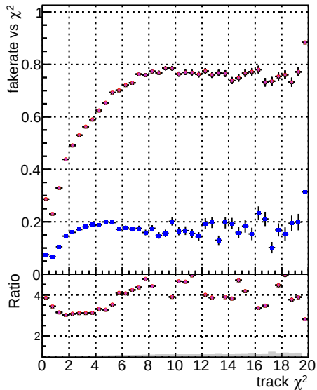
Fake rate vs. \chi^2 for DOM, CKE, TThor, TThor-2, and updated new PLDNN-2
