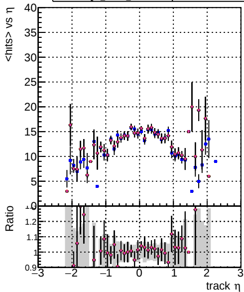
mean hits vs \eta DOM CKE Ttbar DOM mkFit TtbarPU-updated DOM mkFit TtbarPU-updated-newPLDNN-2 DOM mkFit TtbarPU-updated-newPLDNN DOM CKE Ttbar
