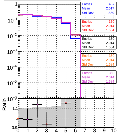
mean hits DOM CKE Tbar DOM mkFit TbarPU-updated DOM mkFit TbarPU-updated-newPLDNN-2 DOM mkFit TbarPU-updated-newPLDNN DOM mkFit TbarPU-updated-TTbarDNN
