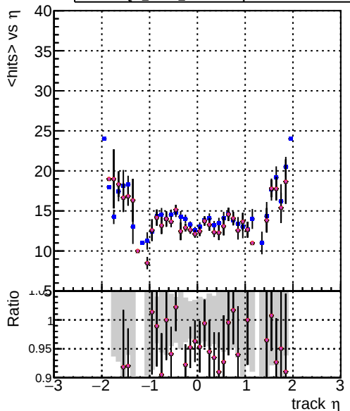
mean hits DOM CKE Tbar DOM mkFit TbarPU-updated DOM mkFit TbarPU-updated-newPLDNN-2 DOM mkFit TbarPU-updated-newPLDNN DOM mkFit TbarPU-updated-TTbarDNN
