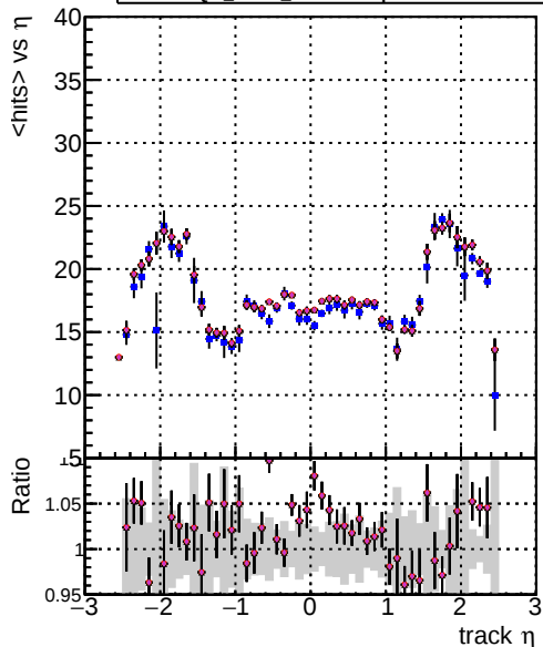
mean hits DOM_CKE_TTbar DOM_mkFit_TTbarPU-updated DOM_mkFit_TTbarPU-updated-newPLDNN-2 DOM_mkFit_TTbarPU-updated-newPLDNN-2 DOM_mkFit_TTbarPU-updated-TTbarDNN
