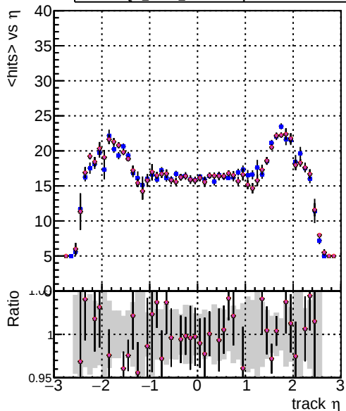
mean hit DOM_CKE_TTbar DOM_mkFit_TTbarPU-updated DOM_mkFit_TTbarPU-updated-newPLDNN DOM_mkFit_TTbarPU-updated-TTbarDNN-2
