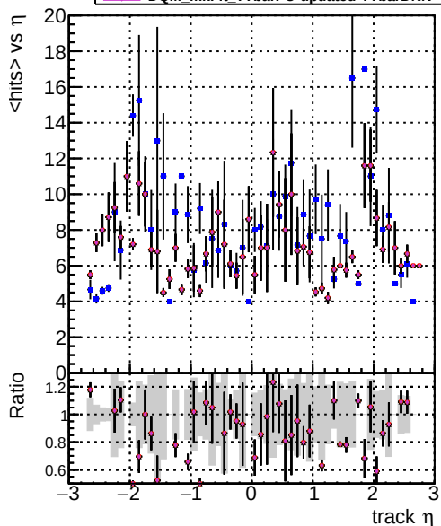
Legend: DOM CKE Tbar, DOM mkFit TbarPU-updated, DOM mkFit TbarPU-updated-newPLDNN, DOM mkFit TbarPU-updated-newPLDNN-2, DOM mkFit TbarPU-updated-TbarDNN mean hits
