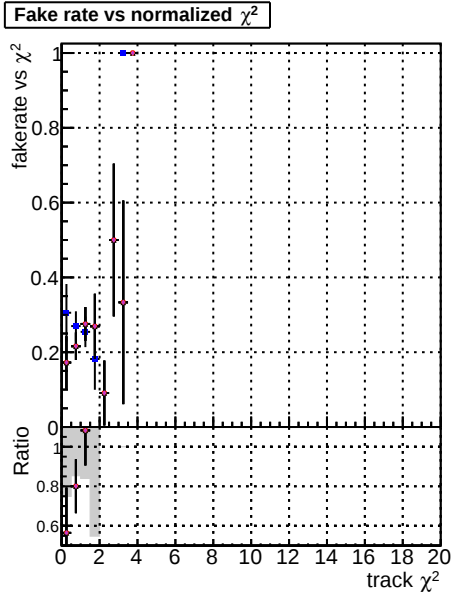
Fake rate vs. DOM CKF TThar TTharBU-updated newPLDNN-2
