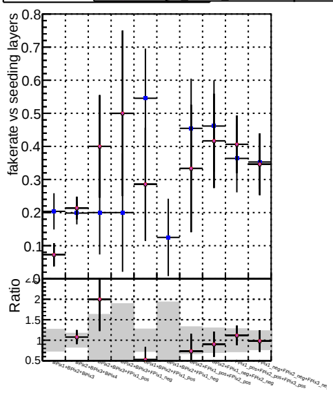
Fake rate vs. DOM CKF TThar TTharBU-updated newPLDNN-2
