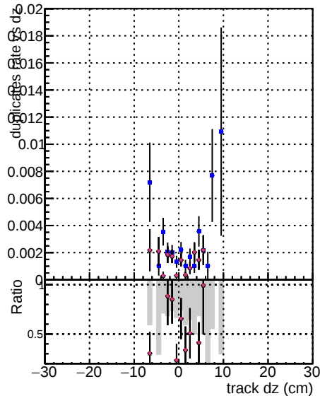
ewBLDNN-2 rbarDNN
