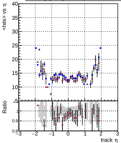
mean hits DOM_CKE_TTbar DOM_mkFit_TTbarPU-updated DOM_mkFit_TTbarPU-updated-newPLDNN-2 DOM_mkFit_TTbarPU-updated-TTbarDNN
