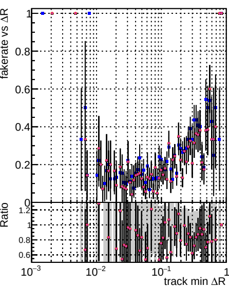
Fake rate vs \Delta R(\text{track, jet}) DQM CKF Tthor PU-updated newPLDNN-2
