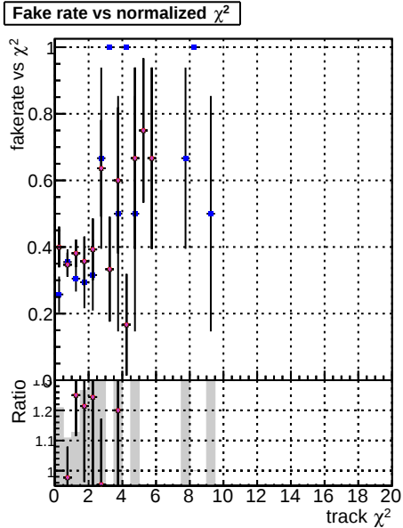
Fake rate vs. \chi^2 Legend: DOM, CKF, TThar, DOM+CKF+TThar, DOM+CKF+TThar+BU-updated, newPLDNN
