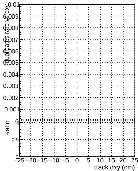
ewBLDNN-2 YbarDNN-2
