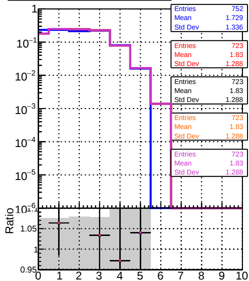
mean hit DOM_CKE_TTbar DOM_mkFit_TTbarPU-updated DOM_mkFit_TTbarPU-updated-newPLDNN-2 DOM_mkFit_TTbarPU-updated-TTbarDNN
