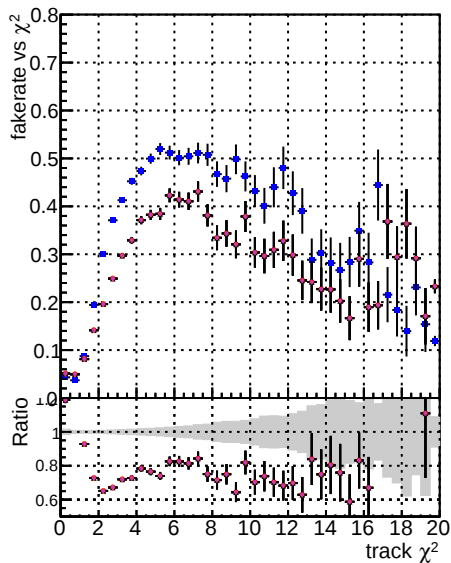
Fake rate vs. DOM GKE TTbar DOM+mkFit TTbar+PU-updated newBLDNN-2 TTbar+PU-updated+TTbarDNN-2
