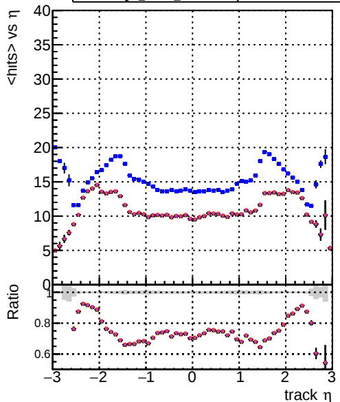
mean hits vs \eta DOM_CKE_TTbar DOM_mkFit_TTbarPU-updated DOM_mkFit_TTbarPU-updated-newPLDNN DOM_mkFit_TTbarPU-updated-TTbarDNN-2
