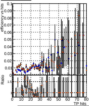
Efficiency vs hit Legend: DQM_CKF_TTbar DQM_mkFit_TTbarPU-updated DQM_mkFit_TTbarPU-updated-newPLDNN DQM_mkFit_TTbarPU-updated-newPLDNN-2
