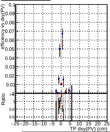
Efficiency vs Dxy(PV) Legend: DQM_CKF_TTbar DQM_mkFit_TTbarPU-updated DQM_mkFit_TTbarPU-updated-newPLDNN DQM_mkFit_TTbarPU-updated-newPLDNN-2
