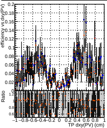
Efficiency vs Dxy(PV) Legend: DQM_CKF_TTbar DQM_mkFit_TTbarPU-updated DQM_mkFit_TTbarPU-updated-newPLDNN DQM_mkFit_TTbarPU-updated-newPLDNN-2
