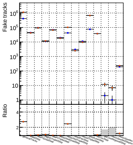
Number —●— DQM_mkFit_TTbar S-updated —★— DQM_mkFit_TTbarPU-updated-newPLDNN —◆— DQM_mkFit_TTbarPU-updated-newPLDNN-2
