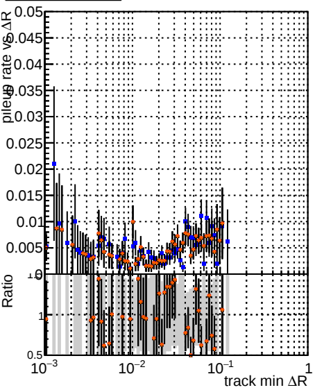
DOM CKE T \bar{T} PU-updated DOM mktfit T \bar{T} PU-updated-new DOM mktfit T \bar{T} PU-updated-newPLBNN-2
