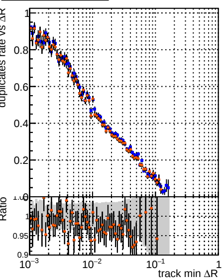
DOM CKE T \bar{T} PU-updated DOM mktfit T \bar{T} PU-updated-new DOM mktfit T \bar{T} PU-updated-newPLBNN-2
