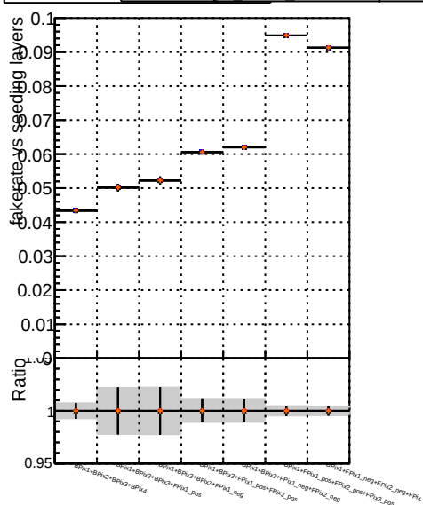
Fake rate vs. DOM GKE TThor DOM MKL TThorPU-Updated-Res PLDNN-2
