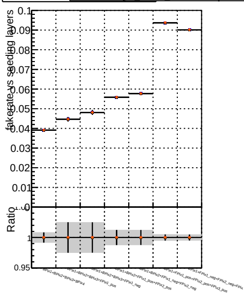
Fake rate vs. DOM GKE TThor DOM MKL TThor DOM MKL TThor-Updated-Res PLDNN-2
