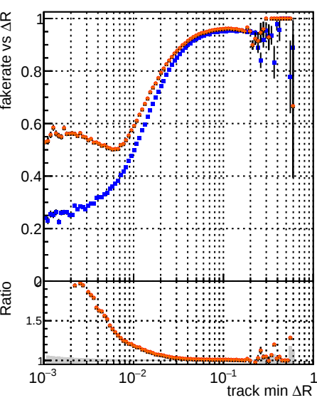
Fake rate vs \Delta R (track, jet) Legend: - DOM CKE Tbar - DOM mktfit Tbar - DOM mktfit Tbar PU-updated - DOM mktfit Tbar PU-updated-new - PLBNN-2
