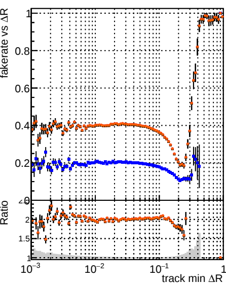
Fake rate vs \Delta R (track, jet) Legend: DOM CKE Ttbar PU-updated DOM mktfit Ttbar PU-updated-new PLBNN-2 DOM mktfit Ttbar PU-updated-new PLBNN-2
