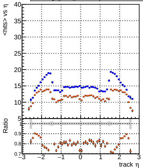
mean hit — DQM_CKFit_TTbar — DQM_mkFit_TTbarPU-updated — DQM_mkFit_TTbarPU-updated-newPLDNN — DQM_mkFit_TTbarPU-updated-newPLDNN-2
