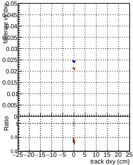
Legend for Fake rate vs dxy: DOM GKE TThor DOM MRIL TThor PU-Updated Revised PLDNN_2
