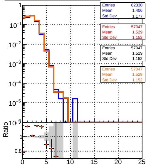
mean hit DQM_CKF_TTbar DQM_mkFit_TTbarPU-updated DQM_mkFit_TTbarPU-updated-newPLDNN DQM_mkFit_TTbarPU-updated-newPLDNN-2
