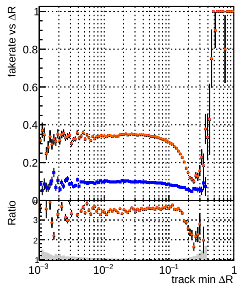
—●— DOM CKE Ttbar —●— DOM mktfit Ttbar —●— DOM mktfit Ttbar PU-updated —●— DOM mktfit Ttbar PU-updated-new PLBNN-2
