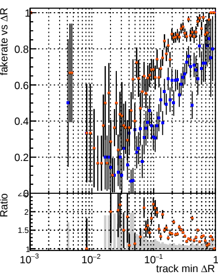
Fake rate vs \Delta R (track, jet) for DOM, CKE, TTbar, PU-updated, and PLBNN-2 models.
