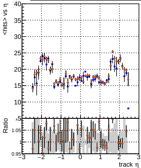
mean hit — DQM_CKFit_TTbar — DQM_mkFit_TTbarPU-updated — DQM_mkFit_TTbarPU-updated-newPLDNN-2 — DQM_mkFit_TTbarPU-updated-newPLDNN-2
