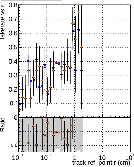
Fake rate vs v Legend: DOM CKE Ttbar PU-updated mkFit TtbarPU-updated mkFit TtbarPU-updated-newPLBNN-2
